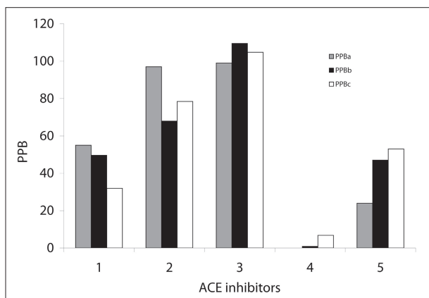
Graph 1. Values of plasma protein binding (PPB) collected from relevant literature (PPBa) [4] and predicted from relation (eq. 1) with calculated \log P_{KOWWIN} (PPBb) or relation (eq. 2) with chromatographic hydrophobicity parameters, C_0 (PPBc)
